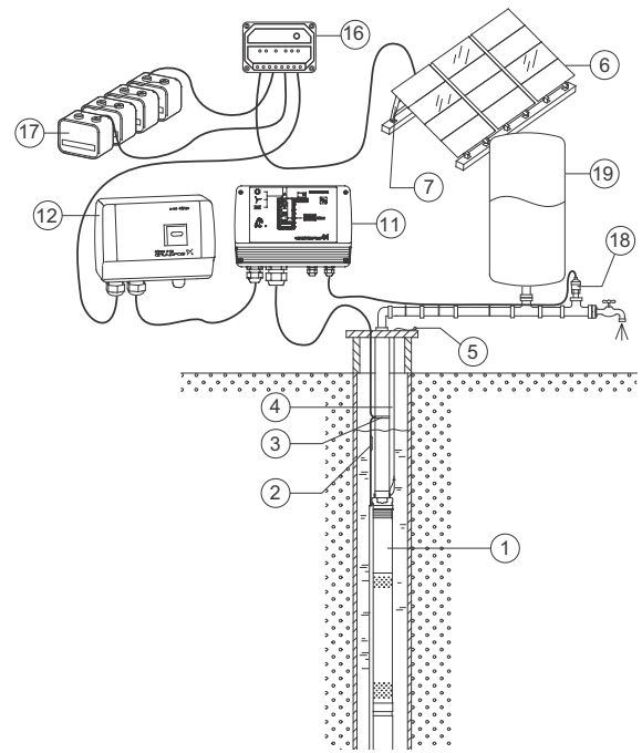
Fig. 10 SQFlex Solar with backup batteries
