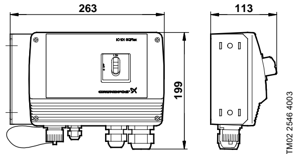
Fig. 25 Dimensions (stated in mm), IO 101
