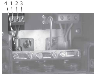
Fig. 5 GENIbus connection
