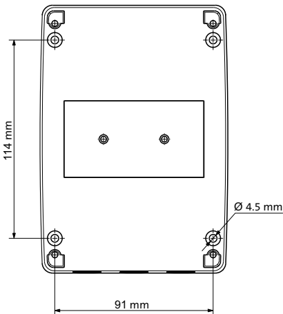
Fig. 2 Wall mounting of the CIU unit
