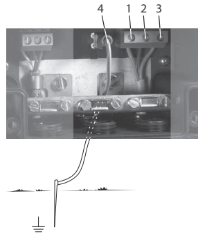
Fig. 4 Electrical connection and earthing
